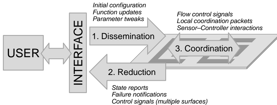
Fig. 4. Computation and communication flows in SDMs.
