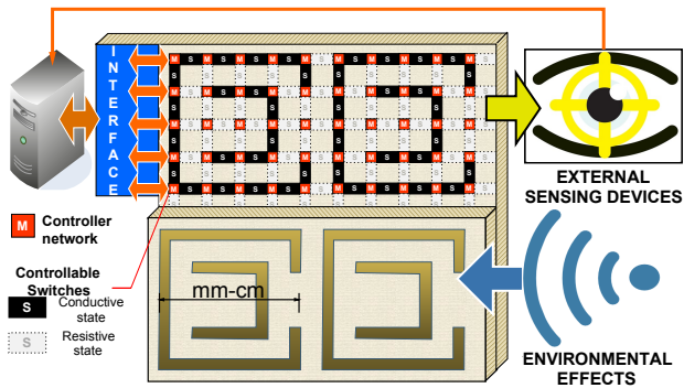
Fig. 1. Schematic representation of a Software-Defined Metamaterial (SDM). External devices drive a network of controllers, whose local decisions determine the global behavior of the metamaterial.
