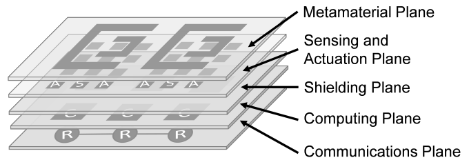
Fig. 2. Sketch of the logical structure of an SDM. It may include actuators (A), sensors (S), controllers (C) and routers (R).
