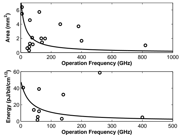
Fig. 6. Area and energy scalability of chip-scale wireless transceivers (data and fitting from [41]).
